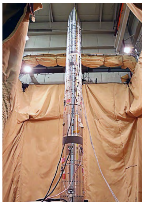
Figure 38: Spin Deployment Facility
