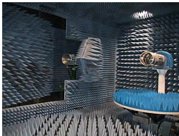
Figure 7: Anechoic Chamber Facility Compact Range Source Feed
