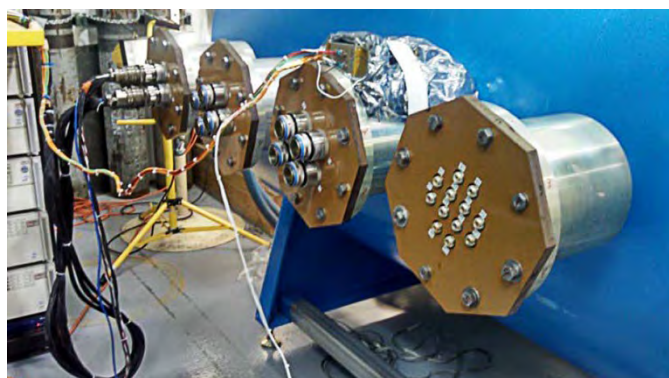
Figure 19: Thermal Vacuum Chamber Ports
